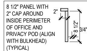
TRIM DETAIL
